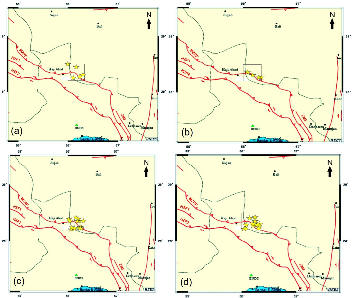
Fig. 7 Distribution of earthquakes in studied region; (a) pre-2000, (b) 2000 to 2006, (c) 2006 to 2008, (d) 2008 to 2023 periods (For the maps used IEES platform)
