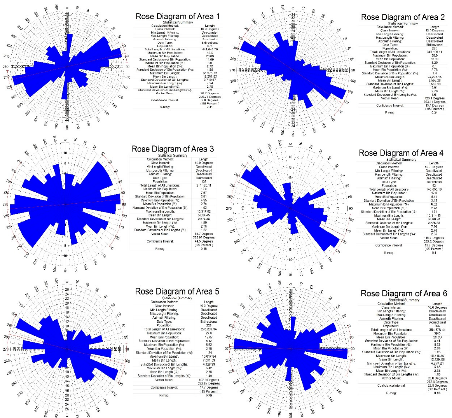
Fig. 6 Rose diagrams for various zones that has been identified in studied region
